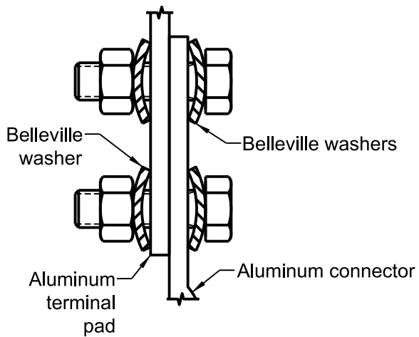
DETAIL A for aluminum-to-aluminum connections
