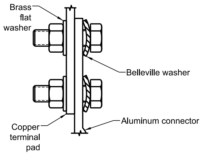
DETAIL D for copper-to-aluminum connections
