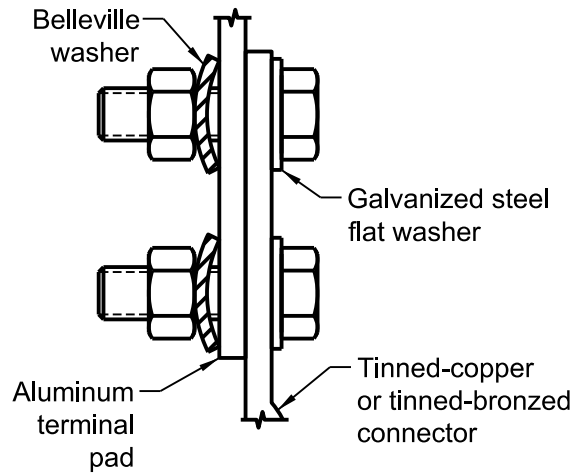
DETAIL B for aluminum to tinned-copper or tinned-bronze connections
