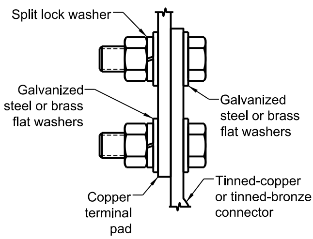
DETAIL C for copper to tinned-copper or tinned-bronze connections
